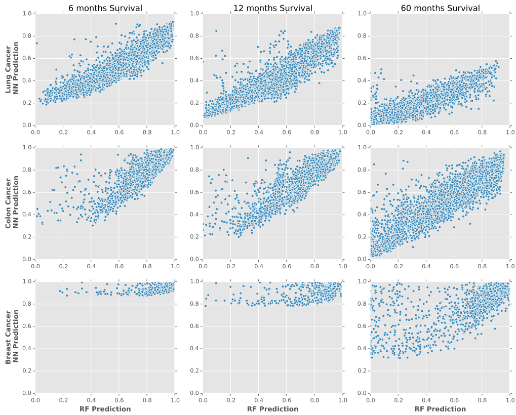
Figure 2. Scatter plots showing the correlations between the MLP model's prediction and RF model's prediction for the probability of surviving at least 6, 12, and 60 months for the lung, colon and breast cancer test data.
